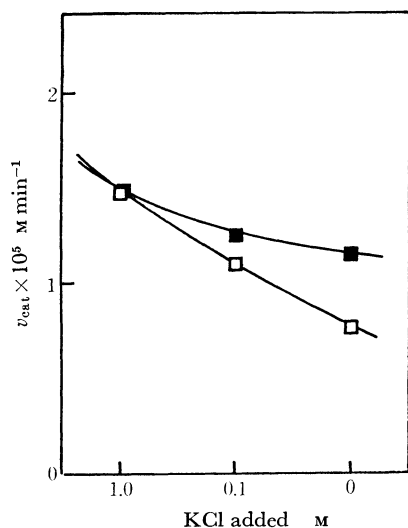
Fig. 5. Effect of ionic strength on catalytic rate.
